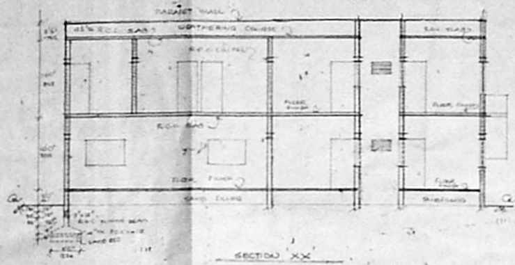
SECTION XX
